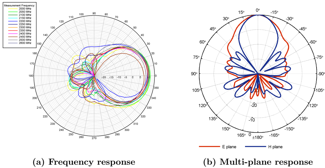
Figure 42. Asymmetric antenna gain properties
