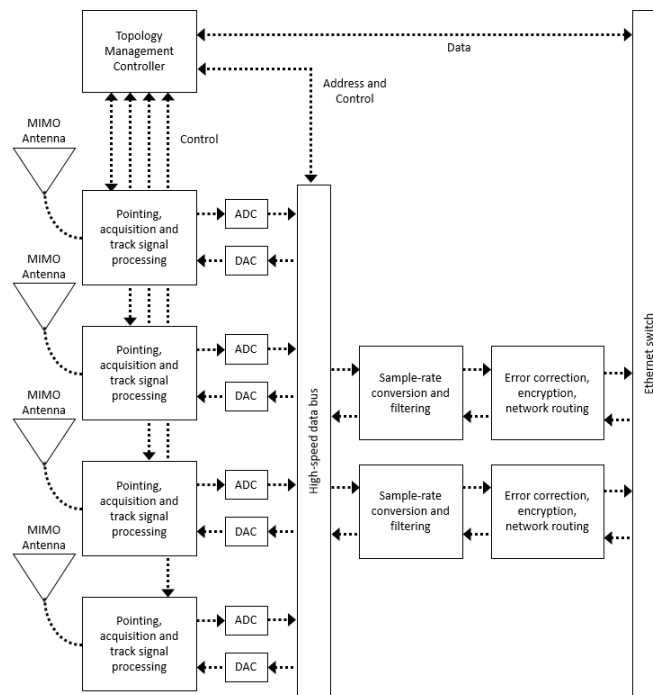
Figure 1. MRA example: four sectors; two transceivers
