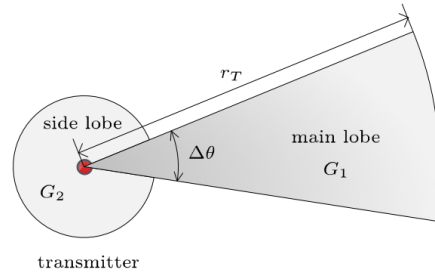
Figure 15. Direction antenna pattern model by [69]
